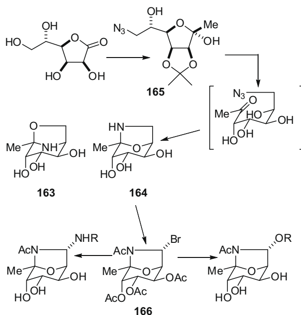
Scheme 34.
