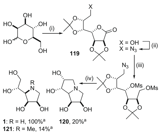
Scheme 23. a Percentage inhibition of lysosomal Golgi human liver \alpha -D-mannosidase at 1 mM concentration.
