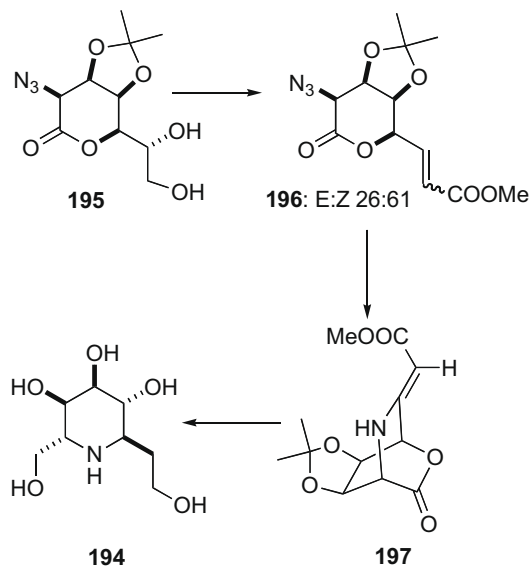
Scheme 40.
