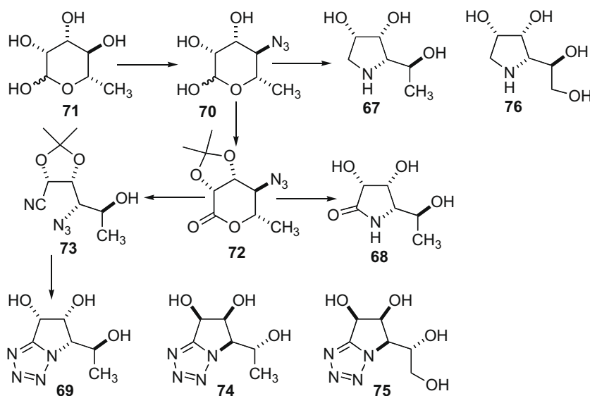
Scheme 15.
