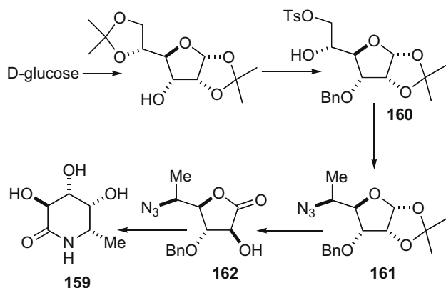
Scheme 33.
