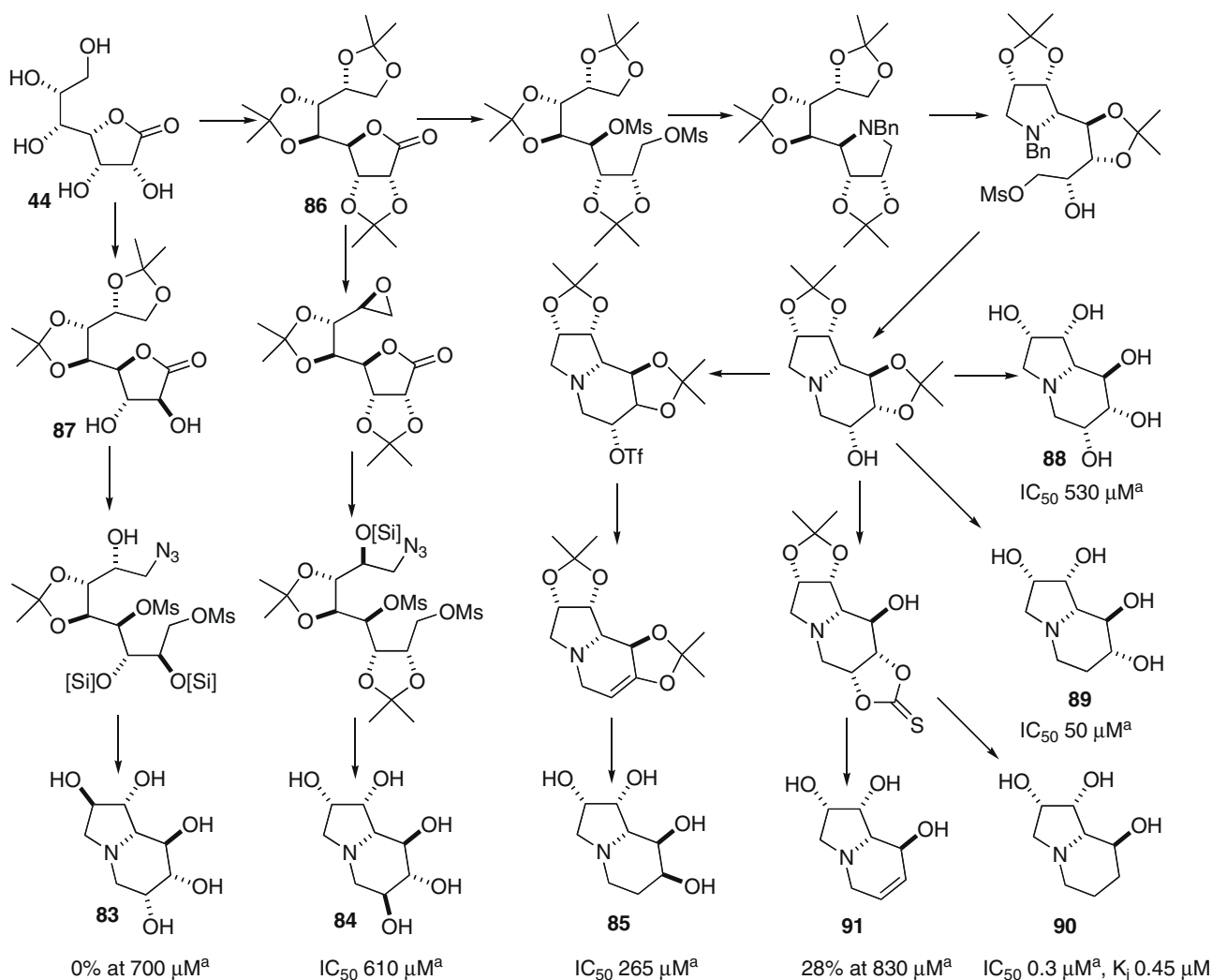
Scheme 17. a Inhibition of naringinase ( \alpha -L-rhamnosidase from P. decumbens ) activity.
