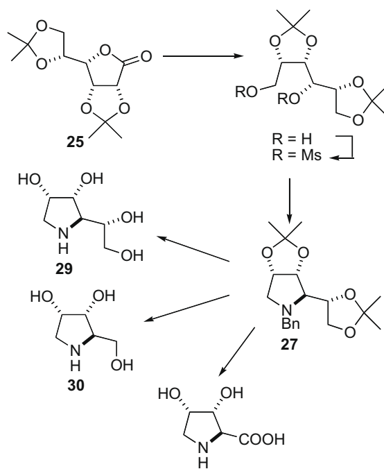
Scheme 7.
