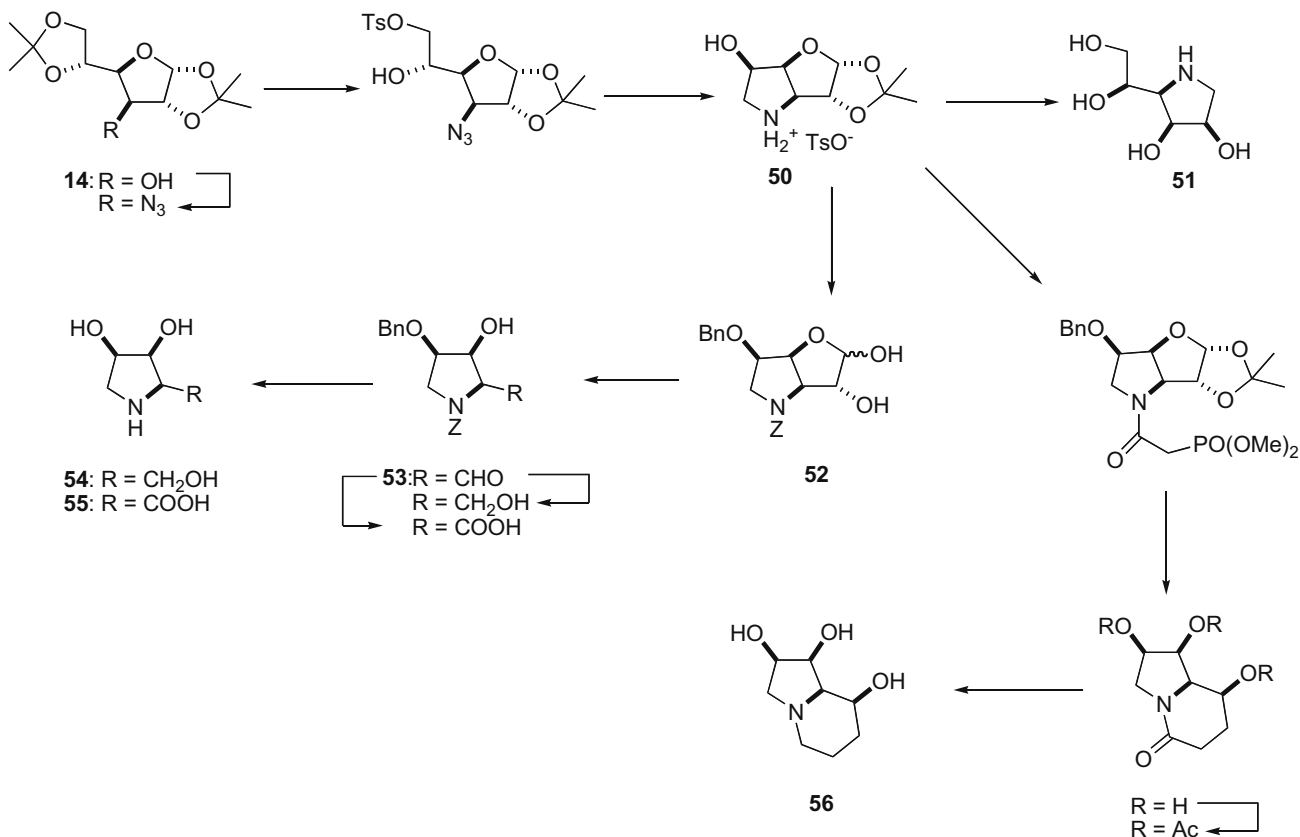
Scheme 11.
