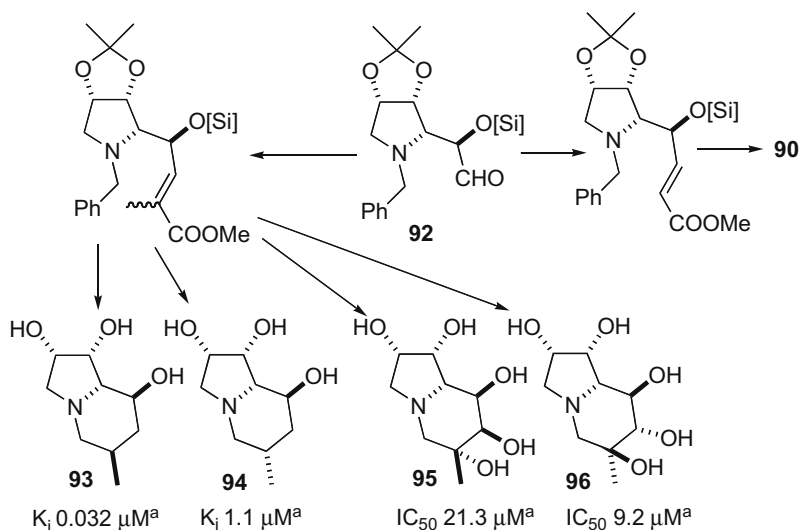
Scheme 18. a Inhibition of naringinase ( \alpha -L-rhamnosidase from P. decumbens ) activity.
