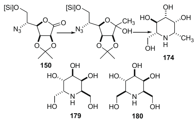
Scheme 38.
