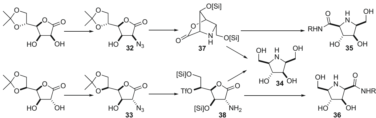
Scheme 8.
