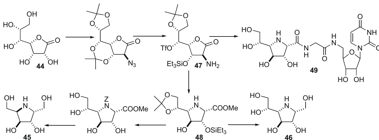
Scheme 10.
