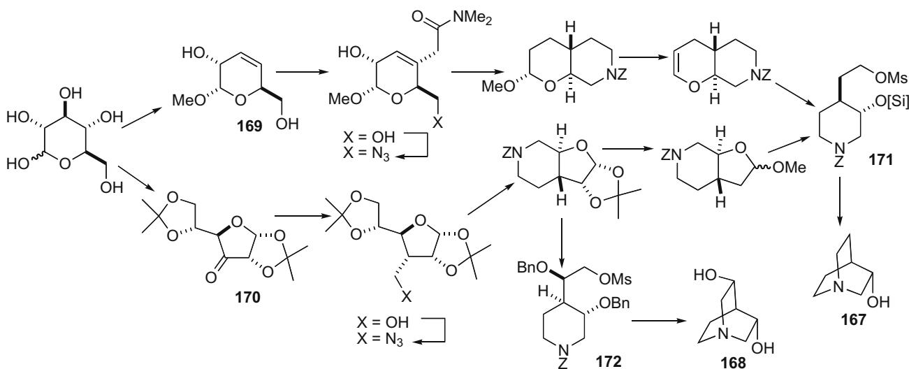
Scheme 36.
