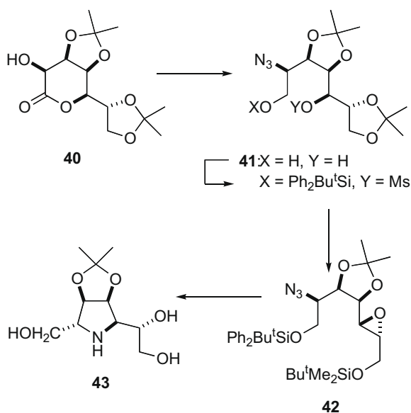
Scheme 9.
