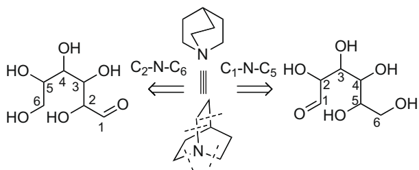
Scheme 35.
