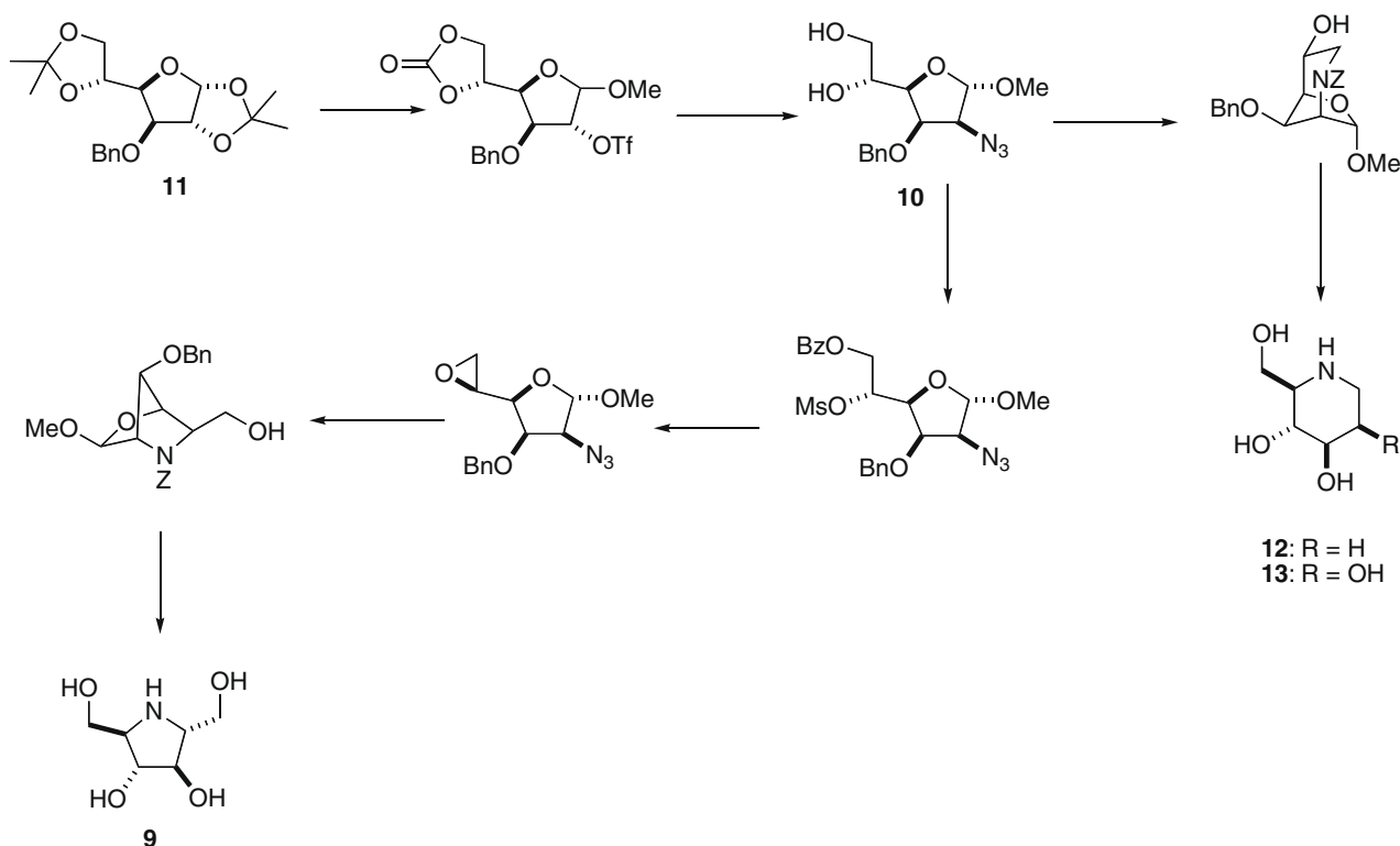
Scheme 3.
