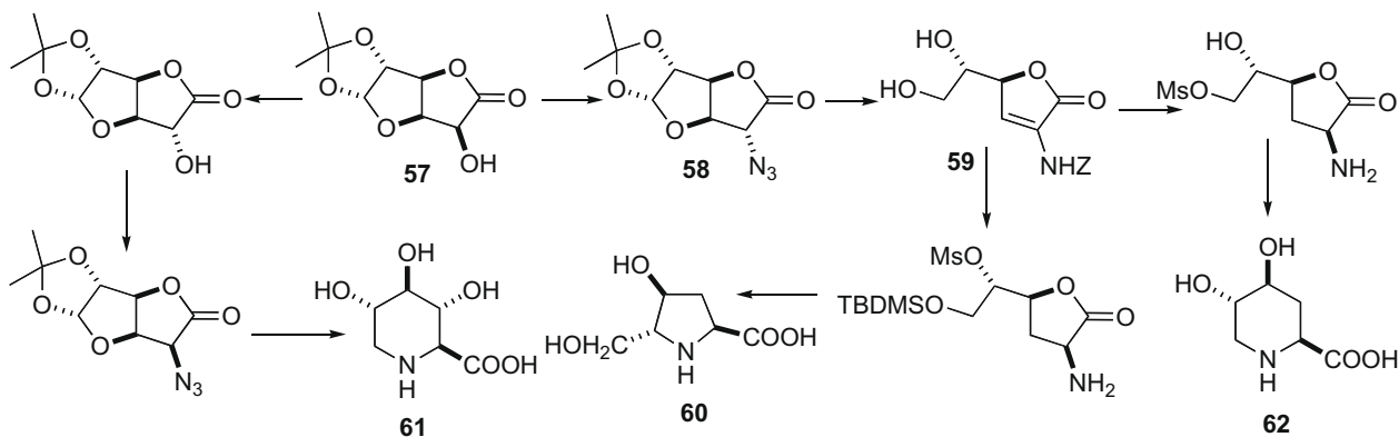
Scheme 13.
